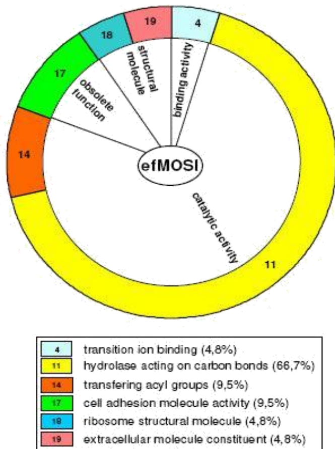
Figure 3. Results of efMOSI GO analysis. The classes and subclasses are represented according to the molecular function category of GOblast tool and the area is proportional to EST sequence number. efMOSI, enriched forward Mirror Orientation Selection library.
