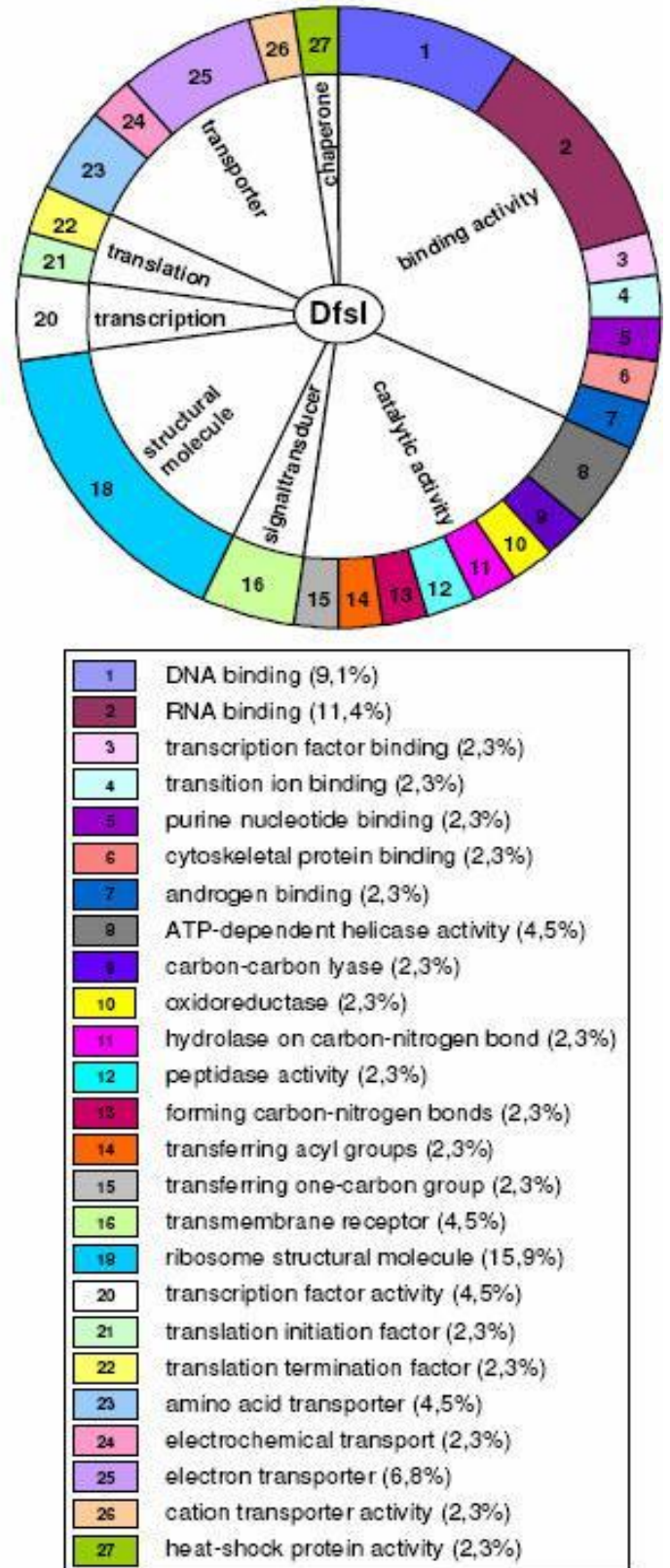
Figure 2. Results of Dfsl GO analysis. The classes and subclasses are represented according to the molecular function category of GOblet tool and the area is proportional to EST sequence number. Dfsl, D irect f orward s ubtractive l ibrary.
