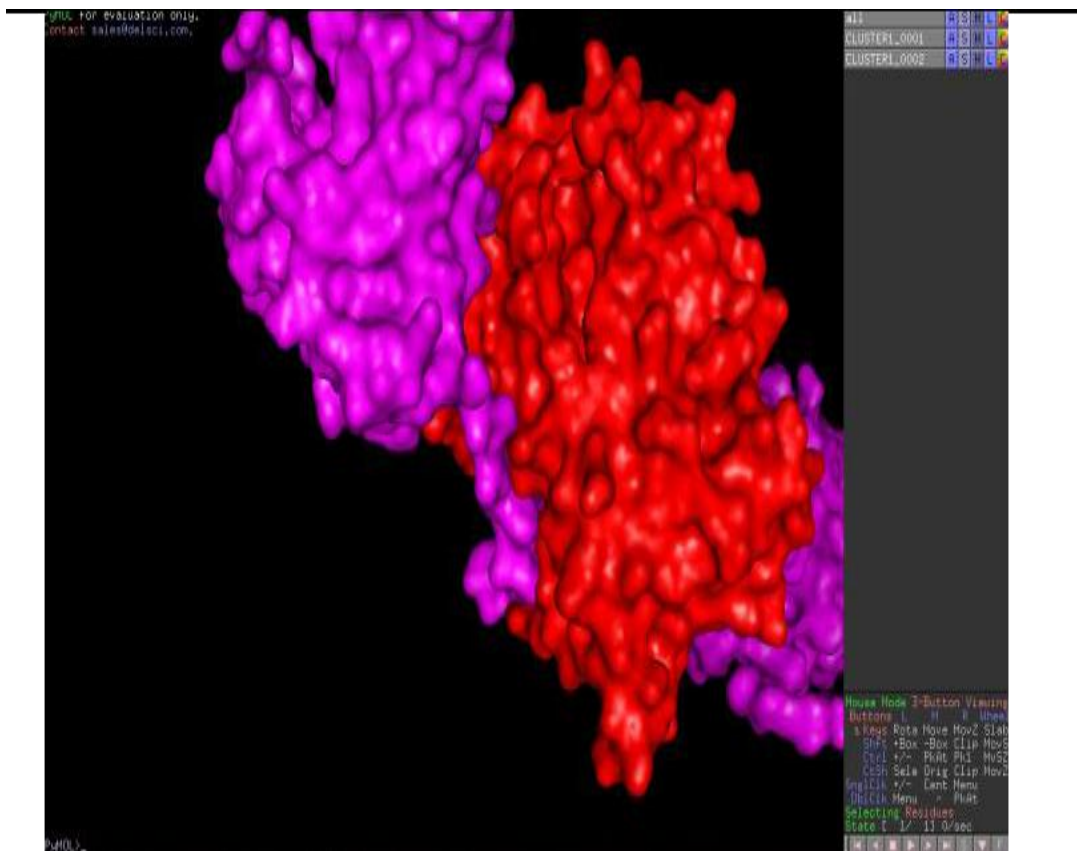
Figure 6. Modified DNMT1 docked with PGC 1 alpha. The two proteins had the interaction with the residues of ARG1187, ARG1181, VAL1189, GLN1212, SER A1149, and SER 225, PHE 226, THR 229, GLY 258, ARG 280. Magenta color = DNMT1; Red = PGC 1 alpha. The ligand molecules are showing the interaction with the active site residues and it has the binding region as in the methyltransferase binding domain.
