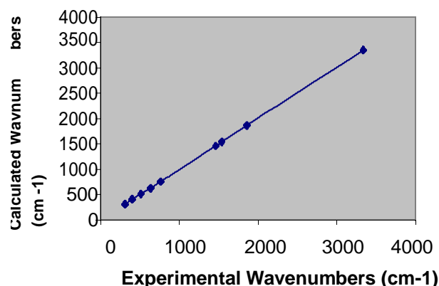
Figure 6. Correlation diagram for experimental Vs calculated frequencies (DFT method) for 3-amino salicylic acid.
