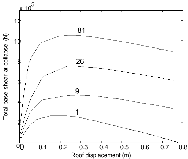
Figure 4. Total base shear for combinations 1, 9, 26 and 81 as a function of roof displacement.
