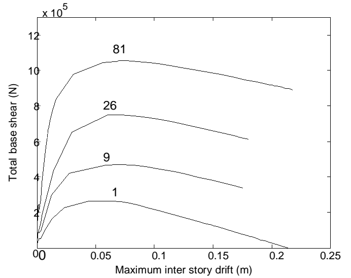
Figure 5. Total base shear for combinations 1, 9, 26 and 81 as a function of maximum inter-story drift.
