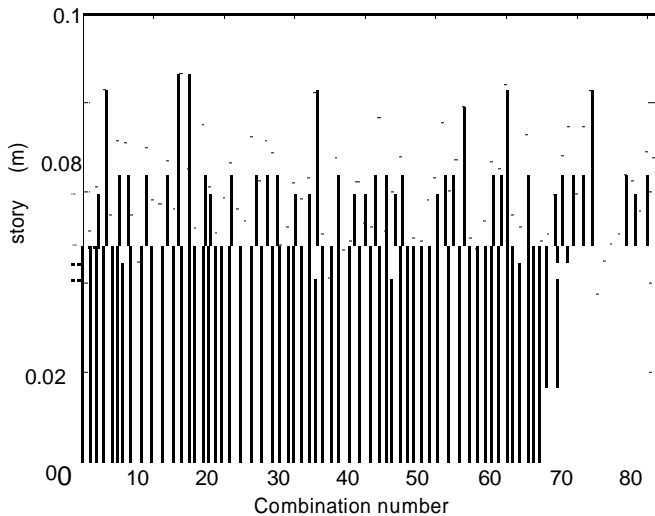
Figure 8. Pushover results in terms of the maximum inter story drifts as function of the combination number.
